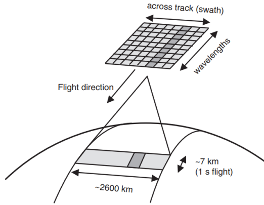
Fig. 2. TROPOMI measurement principle. The dark-gray ground pixel is imaged on the two-dimensional detector as a spectrum. All ground pixels in the 2600km wide swath are simultaneously measured (Veefkind et al., 2012)
